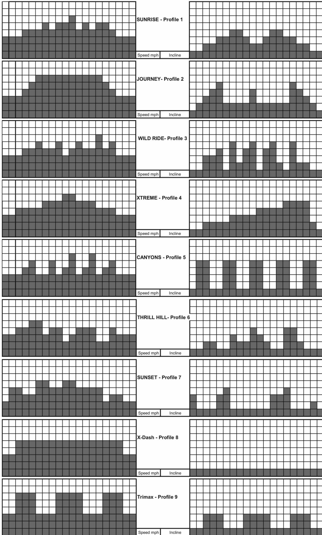
SPEED PROFILE
